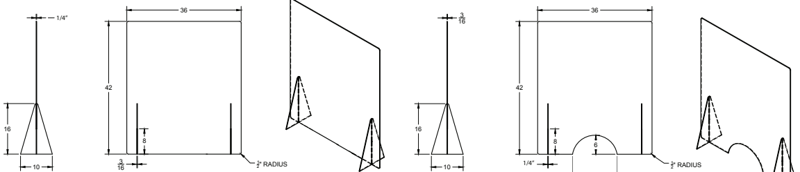
SAFETY SCREEN with pass-through 14" w x 6" h
